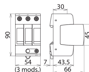
Dimension drawing DG MU 3PY 600 3W+G
