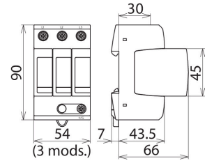
Dimension drawing DG MU 3PY 208 3W+G
